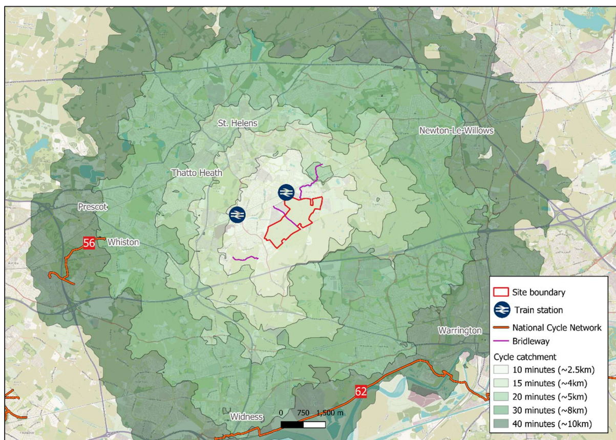
Figure 2.3: Cycling Catchments
