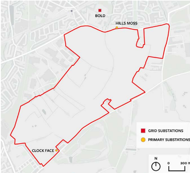
Figure 5.27 Location of the site's local electricity substations.
