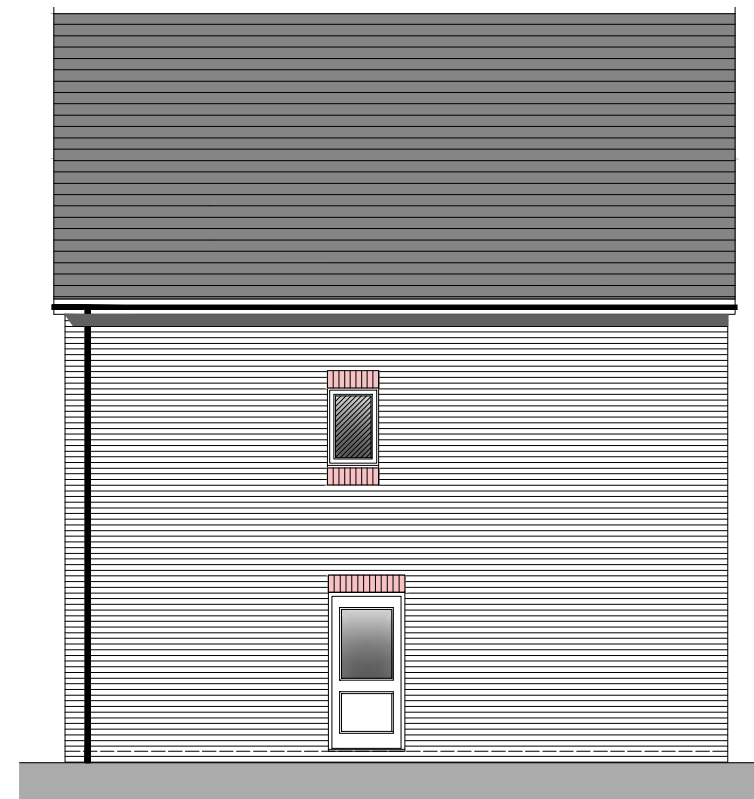
REAR ELEVATION
