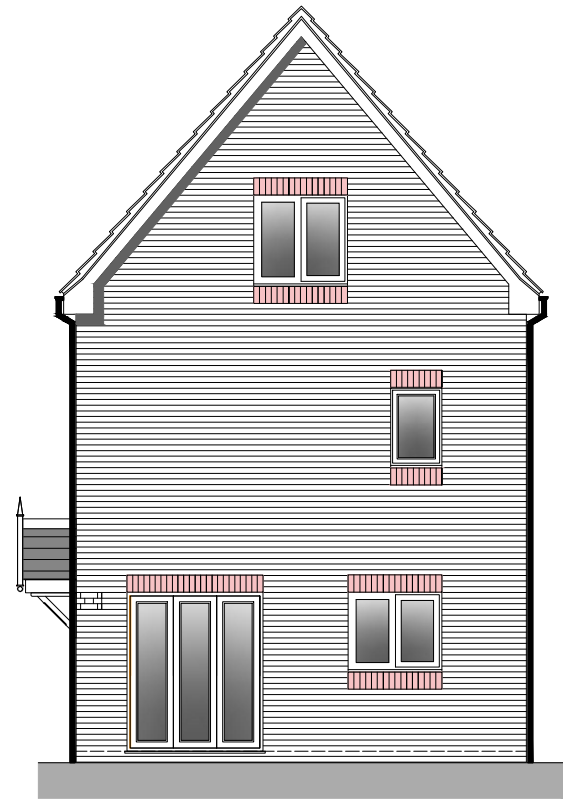
SIDE ELEVATION
