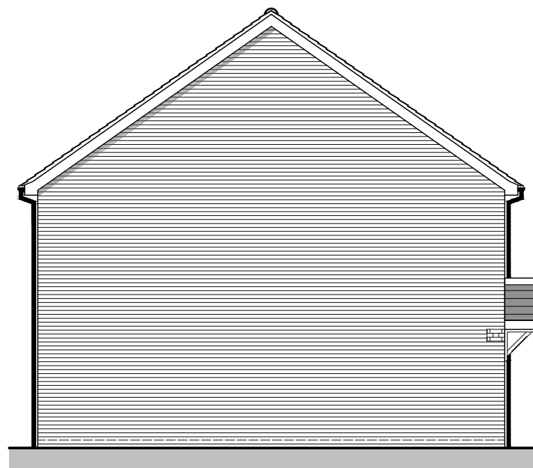
REAR ELEVATION
